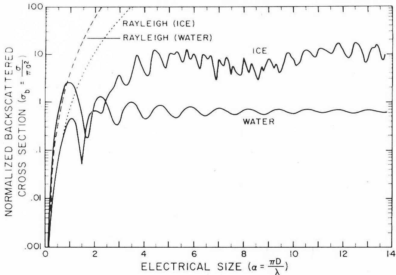
Figure 6.2. Backscatter cross sections for ice and water at 0°C. The Rayleigh approximation is indicated for both cross sections. The electrical size has been determined with a constant wavelength of 10 cm.
