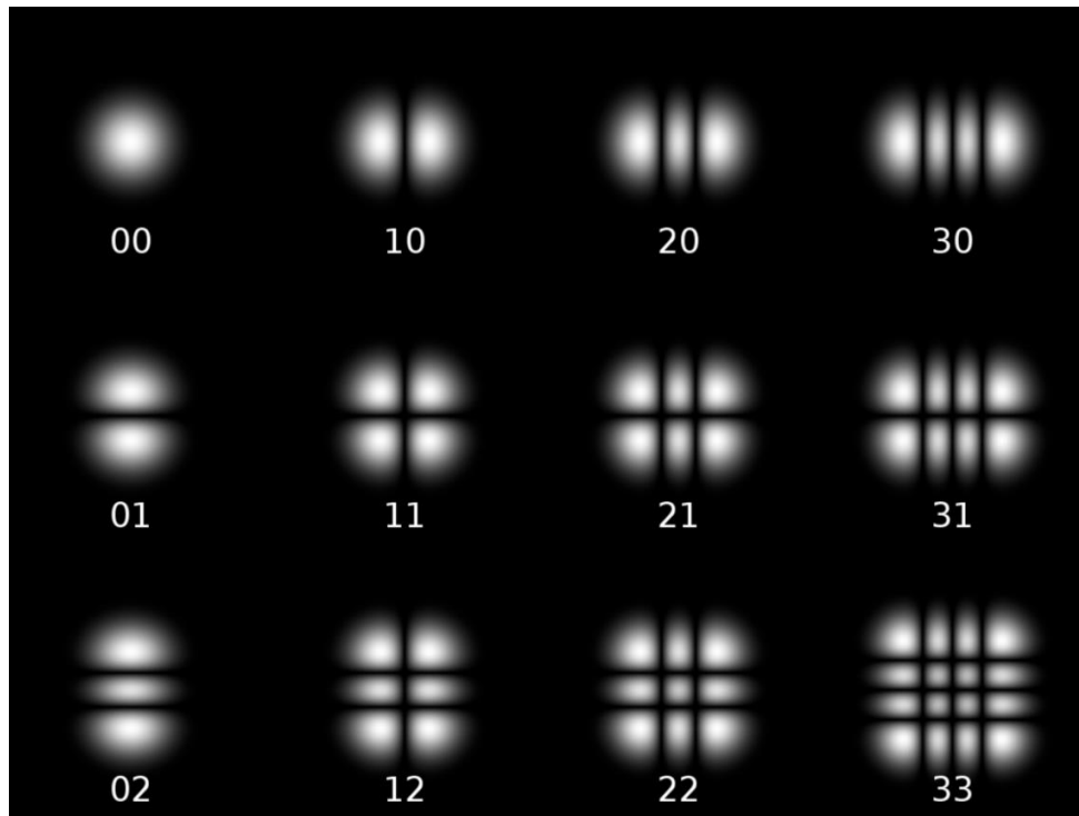
Hermite-Gauss
