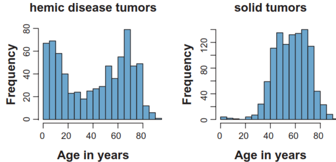
Figure 1. Histogram of the age distribution for the hemic and solid cancer group.
