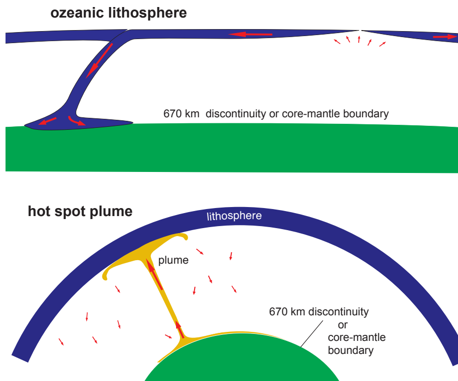
Figure 6.3: The two long-term continuous flow regimes of mantle material-oceanic lithosphere, the one originating at MORs undergoing deep subduction to the 670 km discontinuity or the core-mantle boundary, and the other driven by locally ascending mantle plumes beneath hot spots, are both asymmetric and non-circular.
