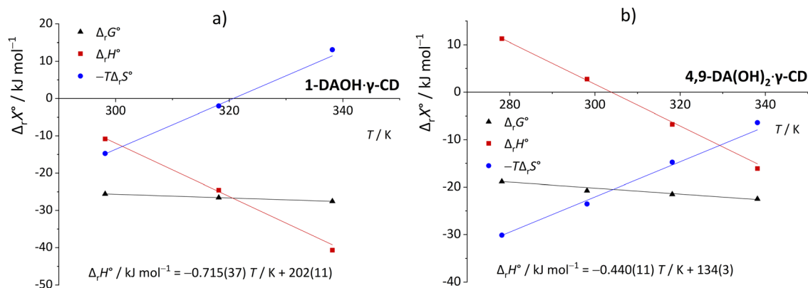
Fig. 6 The temperature dependence of standard complexation parameters of (a) 1-DAOH and (b) 4,9-DA(OH) 2 with \gamma -CD in H 2 O.
